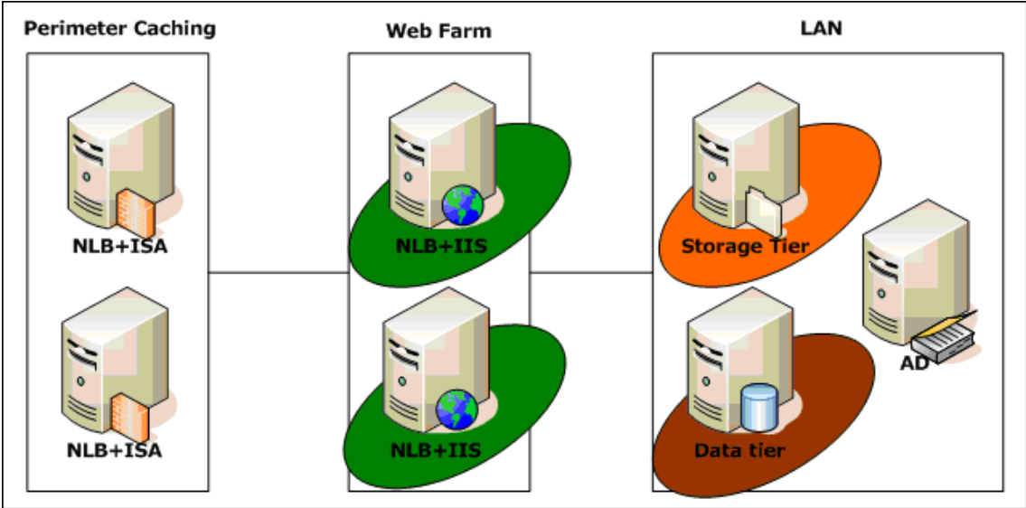
Figure 2: Web Farm
