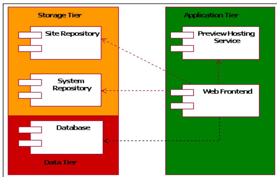
Figure 1: Application components
